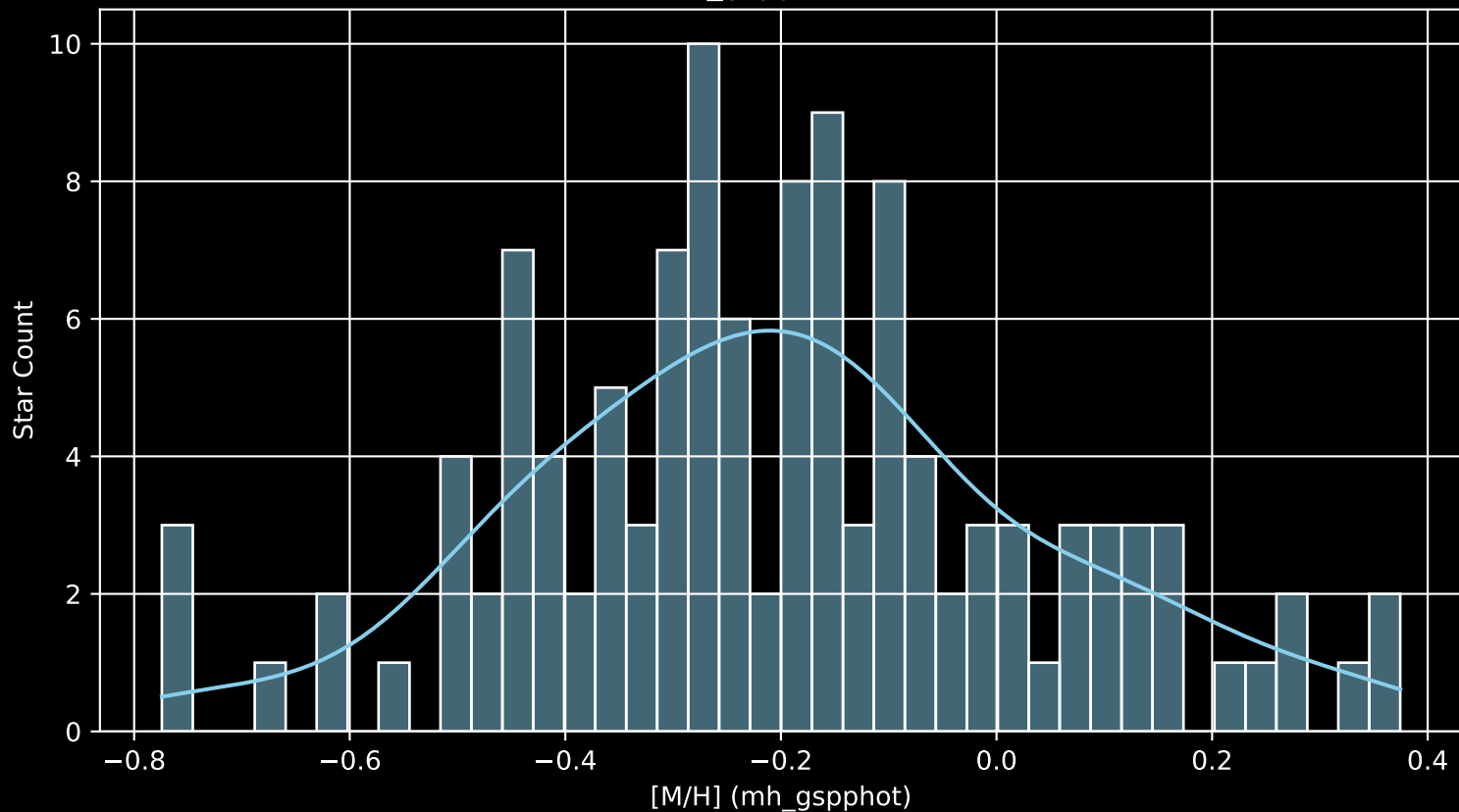
GALAH DR4 Field: [7209] [M/H] (mh_gspphot) (n= 119)
