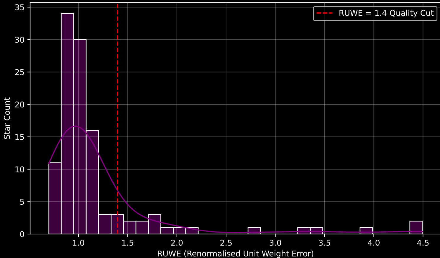
GALAH DR4 Field [7209] RUWE Distribution (n= 113)
