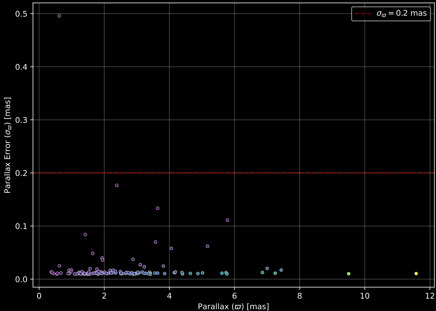
GALAH DR4 Field: [7209] Parallax Quality (n= 119)
