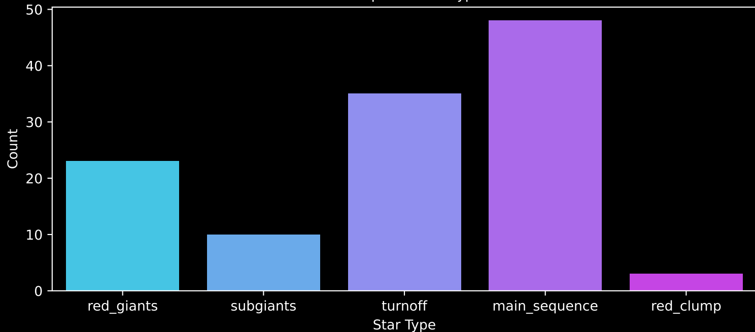
GALAH DR4 Field: [7209] Count plot of Star Type
