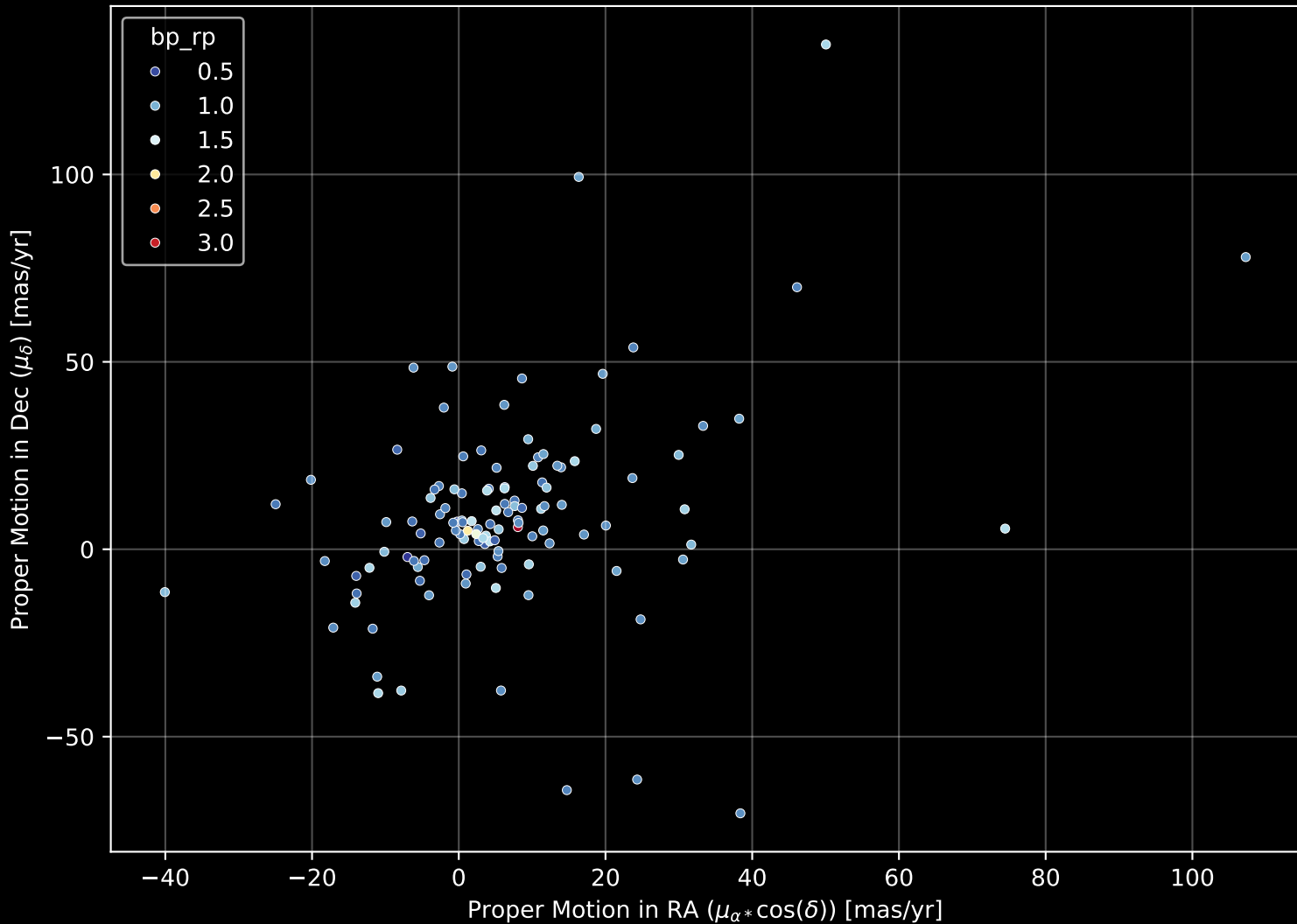
GALAH DR4 Field: [7209] Proper Motion Diagram (n= 119)
